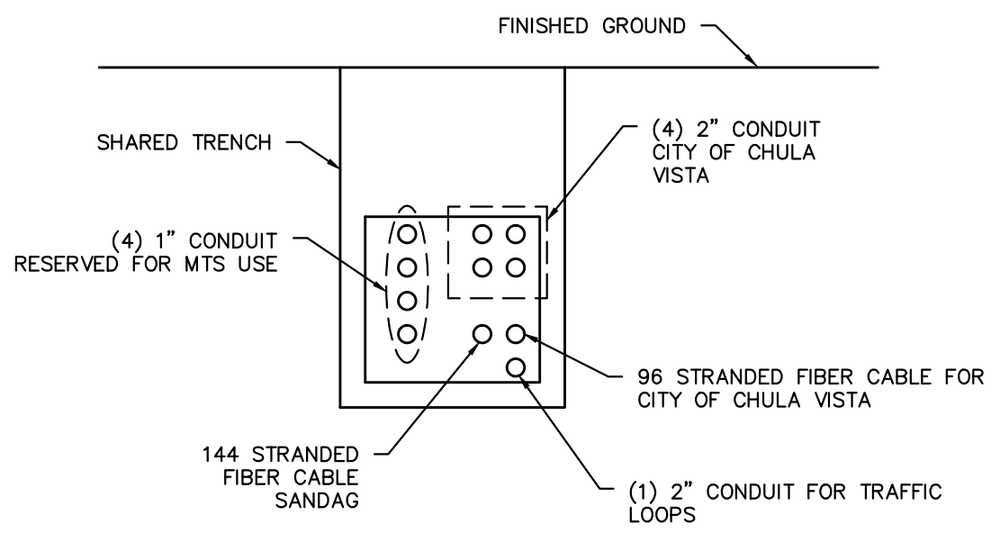
SHARED CONDUIT TRENCH DETAIL FOR ADDITIONAL DETAILS AND TRENCH LOCATIONS SEE SOUTH BAY BRT CONSTRUCTION DRAWINGS
