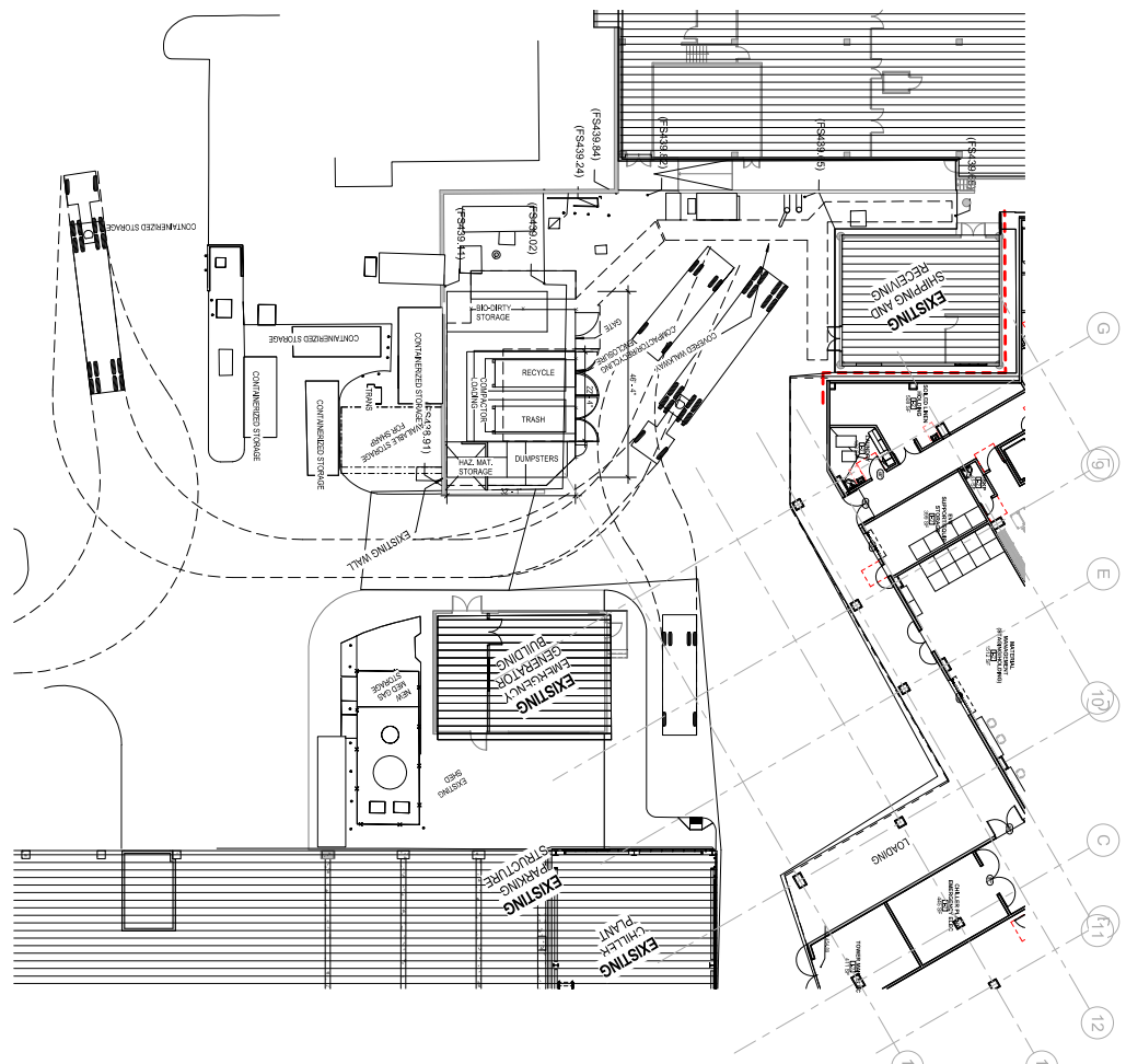
2 OVERALL LEVEL 1 FLOOR PLAN SCALE: 1/8" = 1'-0"
