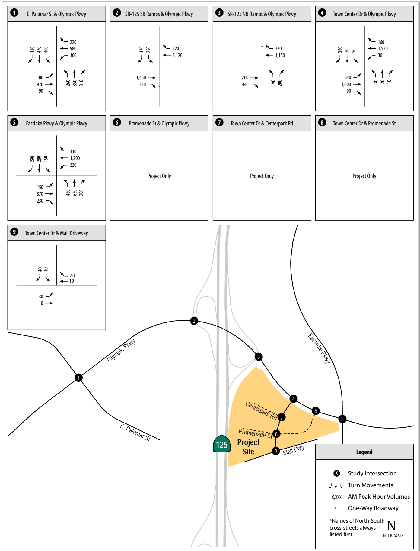
Figure 7 Horizon Year 2030 AM Peak Hour Volumes
